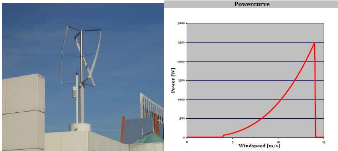
Figure 2.13: The Turby wind turbine and manufacturer's claimed power curve
