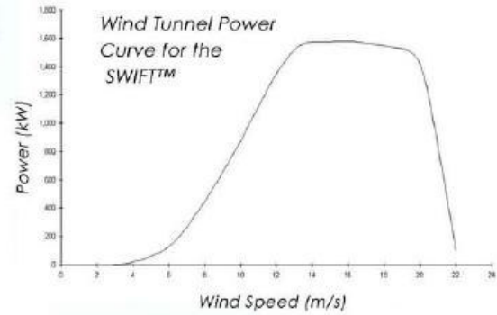
Figure 2.14: The Swift wind turbine and associated power curve
