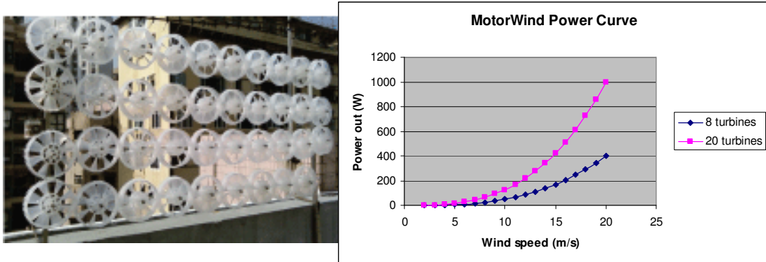
Figure 2.18: MotorWind turbine array and power curve
