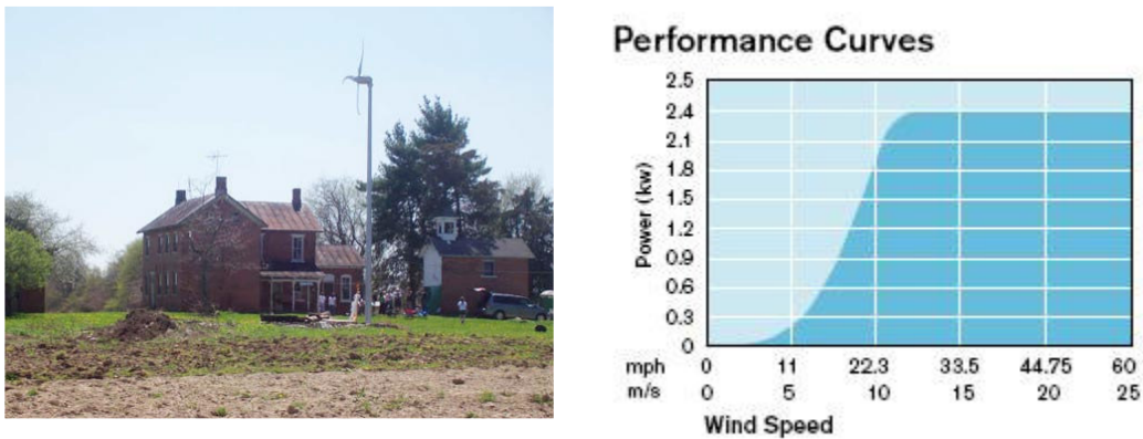
Figure 2.16: Skystream Turbine and power curve
