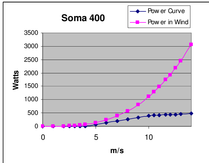
Figure 2.6: Soma 400 Power Curve
