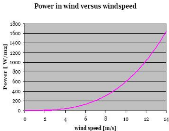
Figure 2.3: Theoretical power in wind
