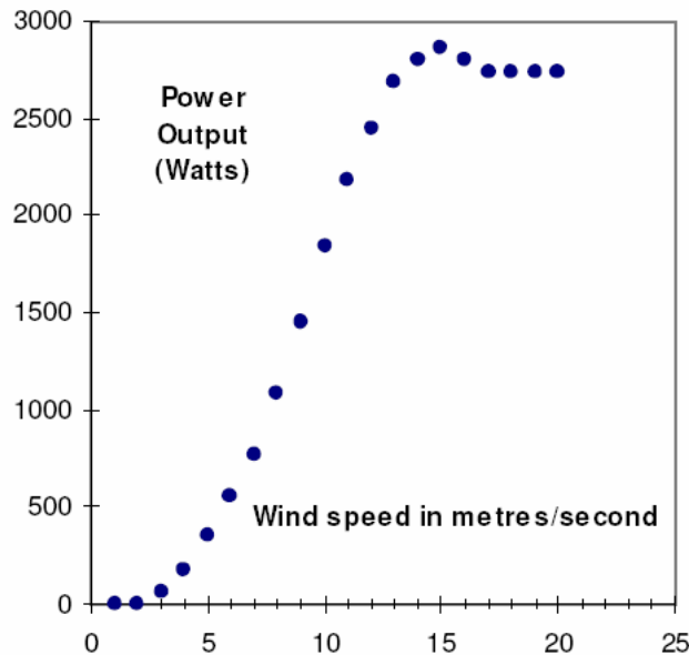
Figure2.4: A typical power curve
